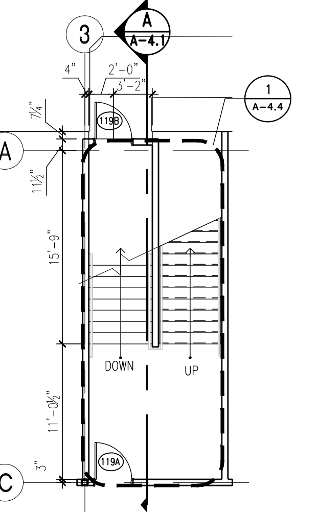
1 LOWER LEVEL STAIR 1/8" = 1'-0"
